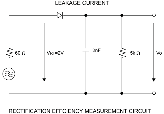
RECTIFICATION EFFICIENCY MEASUREMENT CIRCUIT
