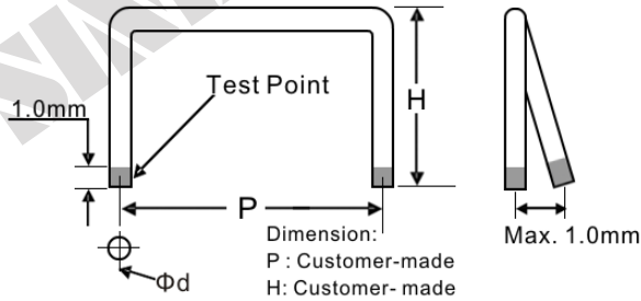
U-Type
