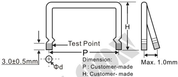
K-Type
