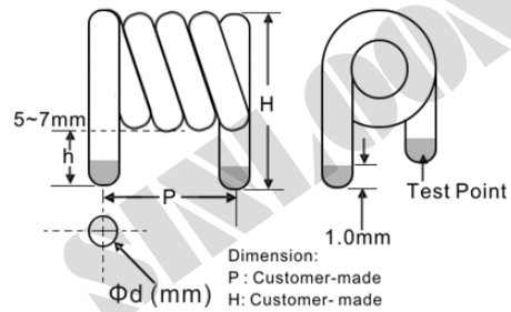
C-Type
