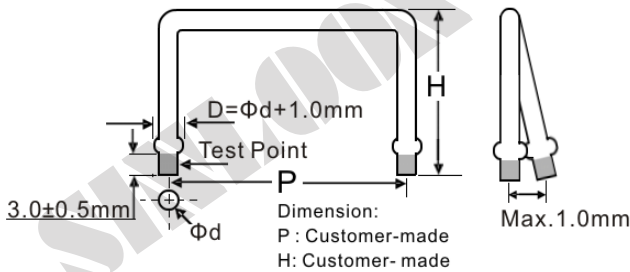
UB-Type
