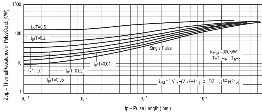
Fig 11. Thermal Response
