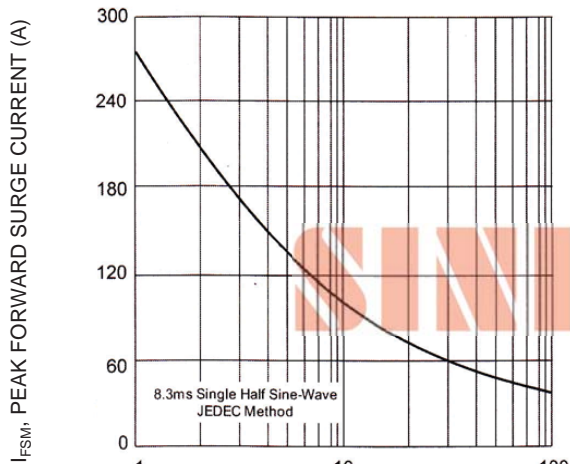
Fig-3 Max. Non-Repetitive Peak Forward Surge Current
