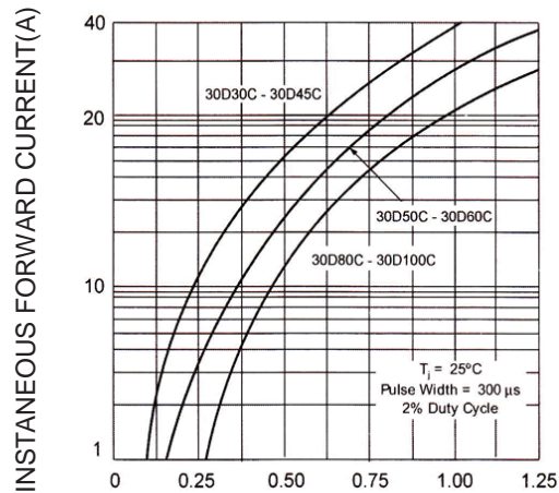
Fig-2 Typical Forward Voltage data per Element.
